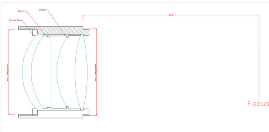
Layout SC Reducer
