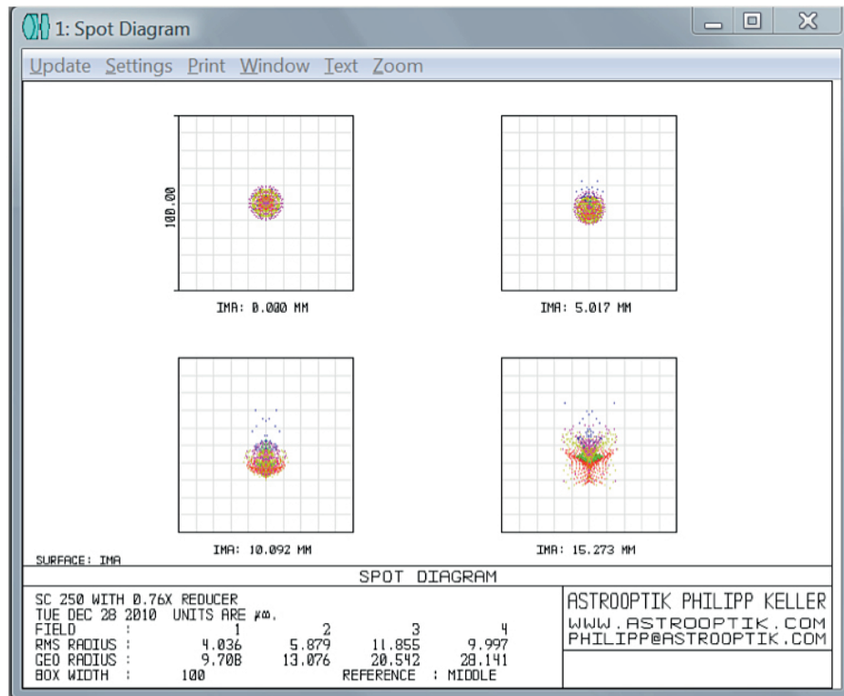
Spotdiagramme SC with ASA 0.77x Reducer Corrector
